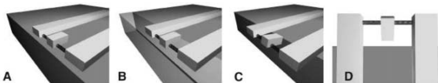
Fig. 1. Principle of sample preparation. (A) The structure is prepared on top of the nanotubes by electron beam lithography close to a cleaved edge of a substrate. (B) An etching process removes part of the substrate. (C) The part of the structure reaching out across the side edge is now free to move. (D) A view from the top shows that it is accessible by the TEM.
